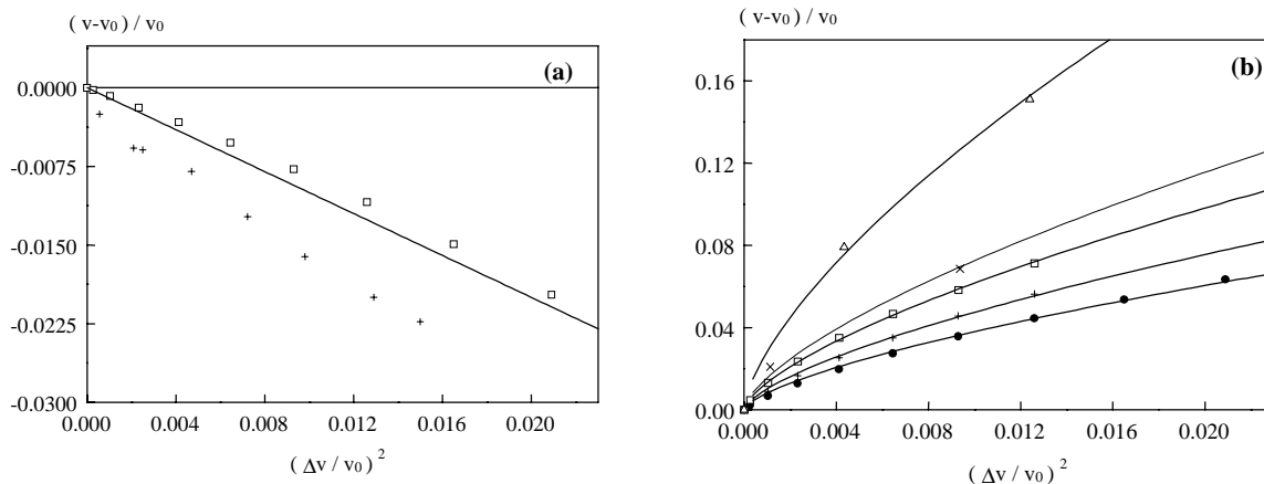
FIG. 2. Dependence of the relative variation in wave velocity vs amplitude disorder both numerically ( \phi_0 = 0.01 ) and experimentally ( T_0 = 3.55 \text{ W/m}^2 ). (a) One-dimensional system. Continuous line (slope -1 ) represents the theoretical prediction of Eq. (7). Numerical points ( \square ) were simulated with stripes of width 10 s.u. (space units) and the best linear fit corresponds to a slope of -0.93 ; experimental data ( + ) were obtained with squares of length of 1.1 cm and adjusted to a line of slope -1.42 . (b) Two-dimensional system. Numerically: for a medium width of 160 s.u. and noise squares of side length 10 ( \bullet ), 20 ( + ), and 40 ( \square ). Continuous lines represent nonlinear fits of Eq. (10), with \beta = 0.831, 1.04, \text{ and } 1.35 , respectively. The typical front width is about 2.5 s.u. Experimental results shown for a medium width of 5.4 cm and l = 2.3 \text{ mm} ( \times ), and for 6 cm and l = 2.7 \text{ mm} ( \triangle ), with \beta = 1.59 \text{ and } 2.89 , respectively. Model parameters: f = 3, q = 0.002, \varepsilon = 0.05, D_u = 1, D_g = 0 , and \phi_0 = 0.01 .
